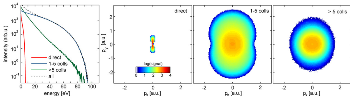
Figure 7. Acceleration-processes-resolved electron energy spectra (a) and projected momentum distributions for 95 nm \text{SiO}_2 particles at an intensity of 3.7 \times 10^{13} \text{ W cm}^{-2} (focus- and CEP-averaged) as calculated with the mean-field Monte-Carlo model. Contributions from direct, backscattered and collisionally heated electrons are determined by exclusively evaluating trajectories without scattering, with up to five scattering events and more than five scattering events, respectively (as indicated).
